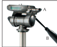
42800 Magnesium Panhead included A Locking screw for 90° side tilt B Vertical movement locking handle
