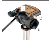
C Integral quick release plate (1/4") with locating pin (removable) D QR plate side locking screw E Locking screw for horizontal panning
