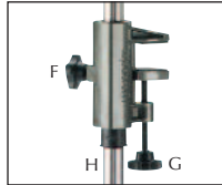
F Centre column vertical movement locking screw G Jaw width adjustment H 500mm centre column
